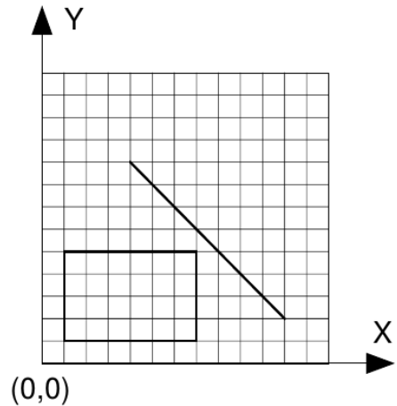
Figure 1: Line segment does not intersect rectangle
